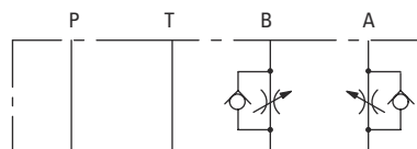
DGMFN-3-Z-T**
