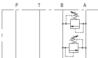
DGMC2-3-AB-**-BA-41
