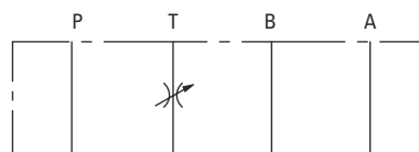
DGMFN-3-Z-T**
