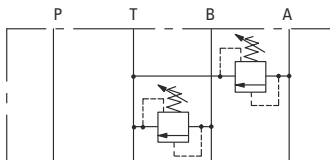
DGMC2-3-AT-**-BT-41
