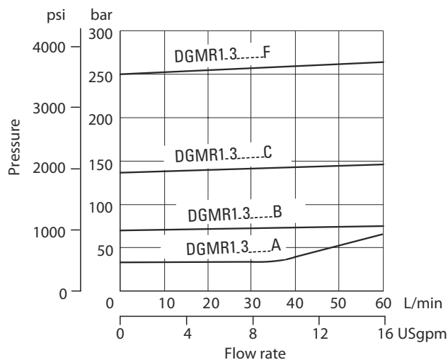
DGMR1-3-PP
