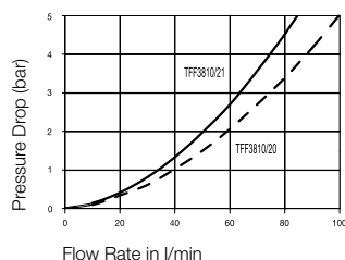
Flow Capacity Viscosity for 32cSt as 40°C as per ISO 7241/2-2000
