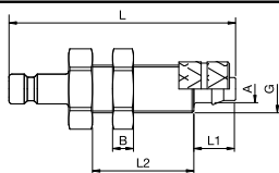
Panel Mount, Plastic Hose Connection
