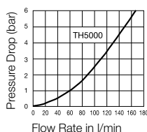
Flow Capacity Viscosity for 32cSt as 40°C as per ISO 7241/2-2000
