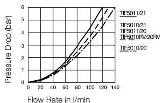
Flow Capacity Viscosity for 32cSt at 40°C as per ISO 7241/2-2000
